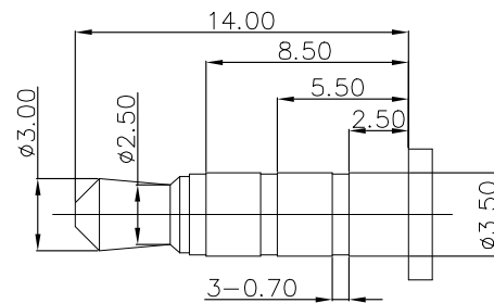
(φ3.50mm 4 POLE PLUG DETAIL DRAWING)
