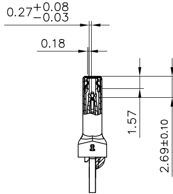
SECTION B-B SCALE 1:1 (WITH EMI SPRING)
