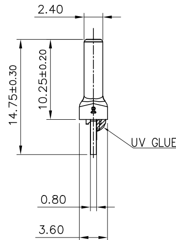
SECTION B-B SCALE 1:1 (WITH EMI SPRING)
