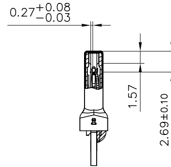
SECTION B-B SCALE 1:1 (WITHOUT EMI SPRING)
