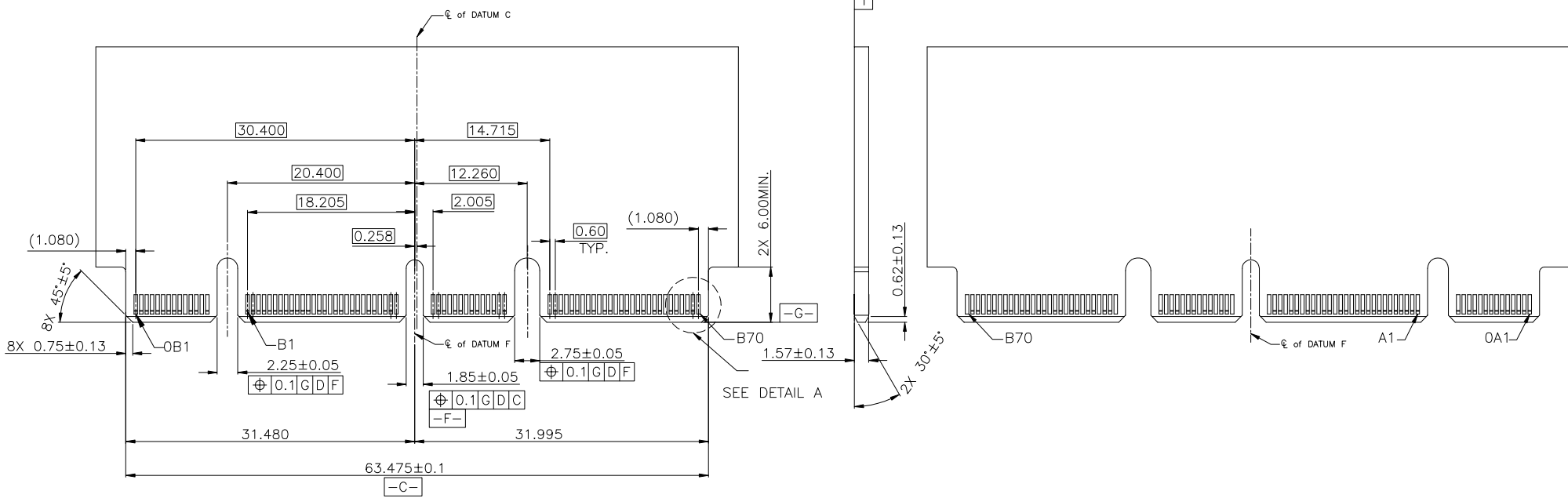
RECOMMENDED AIC 4C+ MATING CARD LAYOUT TOLERANCE ±0.05
