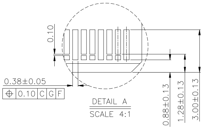
RECOMMENDED AIC 4C+ MATING CARD LAYOUT TOLERANCE ±0.05
