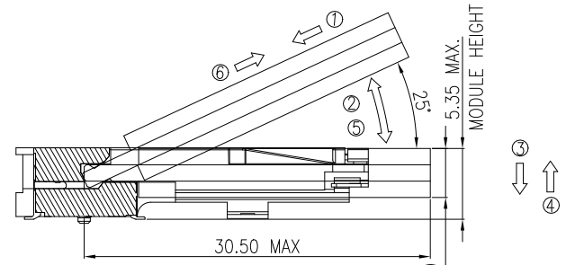
MATING/UNMATING VIEW SCALE 2:1
