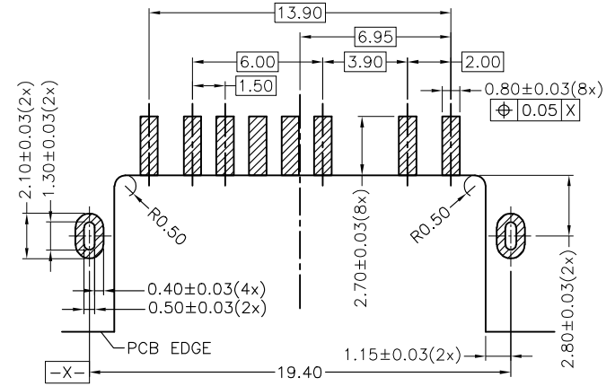
TOP VIEW RECOMMENDED P.C.B LAYOUT TOLERANCE:±0.03mm
